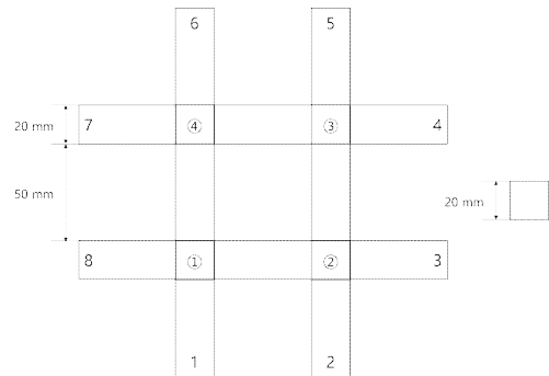
Figure 3. Schematic of electrode placement and k-type thermocouple positions
