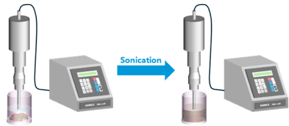
Fig. 1. Cleaning the spent coffee ground using an ultrasonic processor
