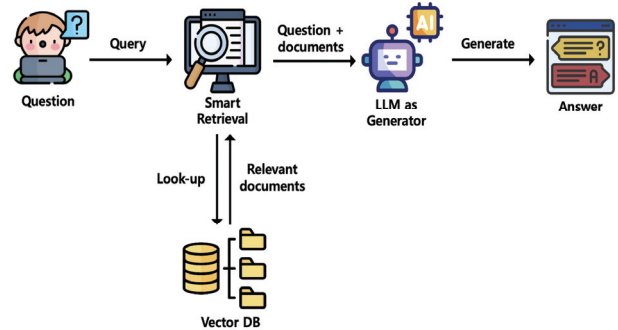
Fig. 1. Architecture of RAG
