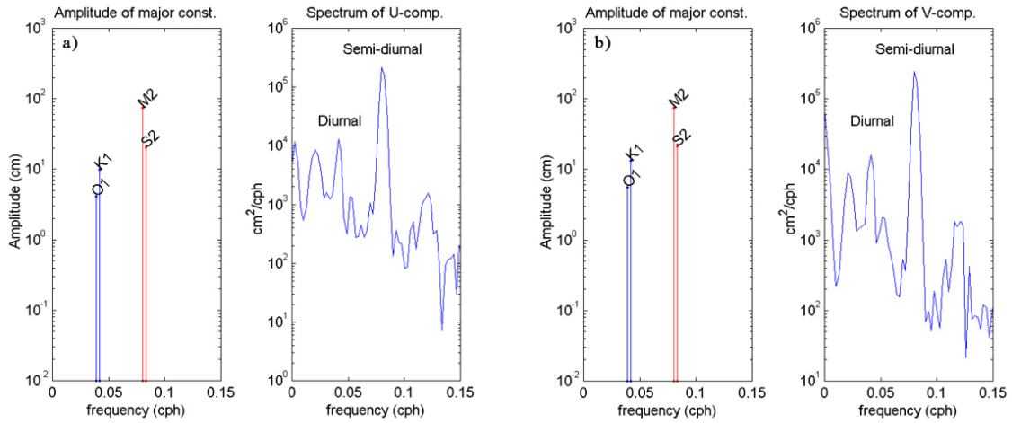
Fig. 4. Results of the harmonic and spectrum analysis for U-comp. (a) and V-comp. (b) of the observed tidal current at Haenam.
