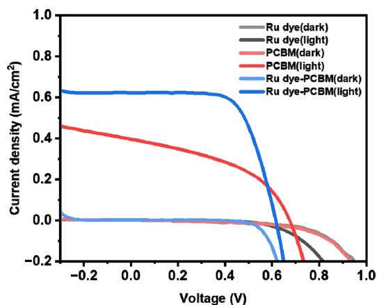
Fig. 8. J–V curves of heterojunction solar cells using blending layer.
