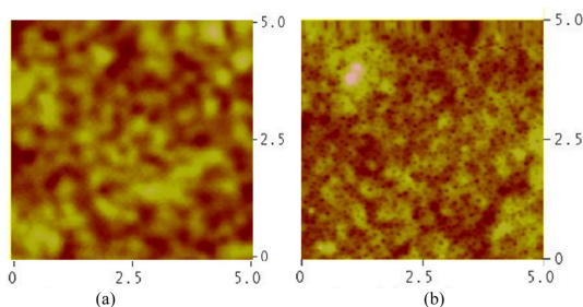
Fig. 7. AFM data of (a) P3OT film and (b) Ru dye-PCBM:P3OT blending film on ITO glass (x-y scale : \mu\text{m} , z scale : nm up to 50 nm).
