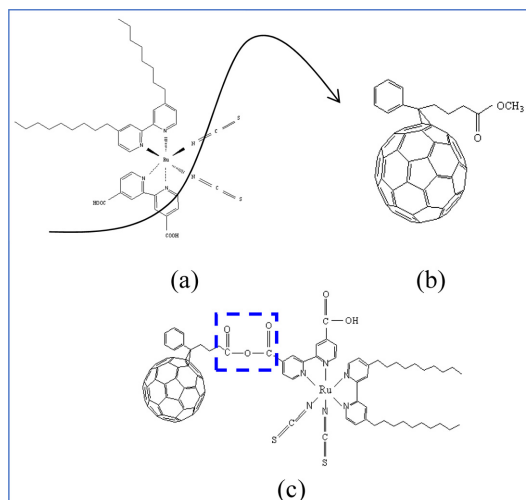
Fig. 1. Synthetic mechanism of Ru dye-PCBM particle. (a) Ru dye (Z-907, Solaronix), (b) PCBM, (c) Ru dye attached with PCBM (Ru dye-PCBM). Rectangle region: anhydride bonding.
