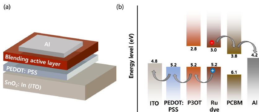
Fig. 6. (a) Structure and (b) energy level of bulk heterojunction solar cells using Ru dye-PCBM particles.
