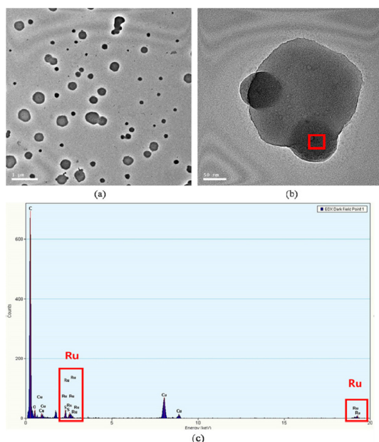
Fig. 4. (a, b) TEM data and (c) EDX of Ru dye-PCBM particle (red region in (b)).
