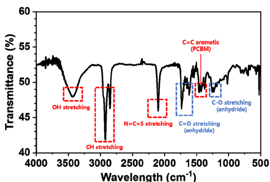
Fig. 2. IR spectra of Ru-dye-PCBM particles.
