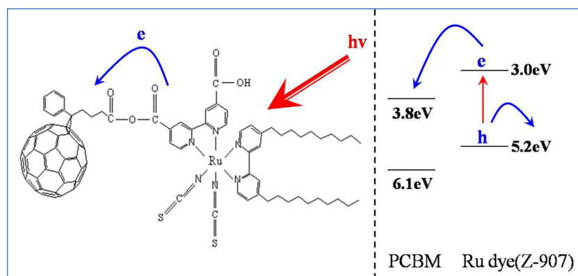
Fig. 5. Schematic of charge transfer in Ru dye-PCBM particles.
