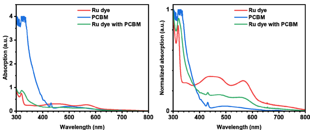
Fig. 3. UV-Vis absorptive spectra of Ru dye-PCBM particles.
