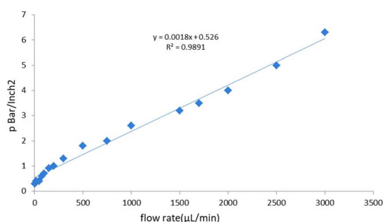
Fig. 4. The relationship between pressure and flow rate.
