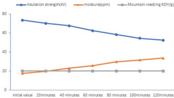
Fig. 3. Measurement graph by the elapsed time at 70% humidity.
