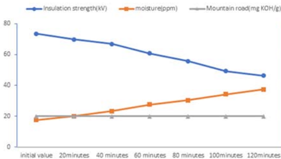
Fig. 4. Measurement graph by the elapsed time at 80% humidity.
