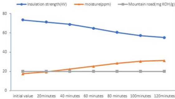
Fig. 2. Measurement graph by the elapsed time at 60% humidity.
