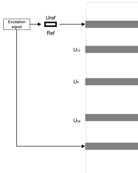
Fig. 2. Schematic diagram of a conductivity longitudinal sensor for crude oil moisture content measurement.
