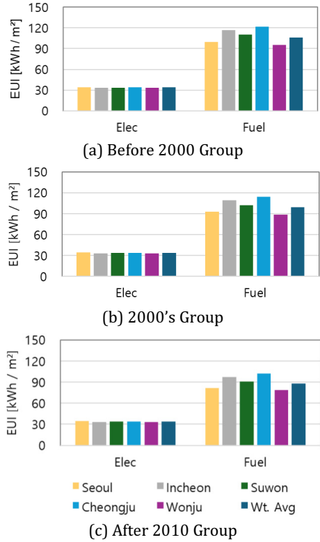
Fig. 4. Annual Electricity and Fuel EUI of Calibrated APT Model Per Vintage for Central Zone
