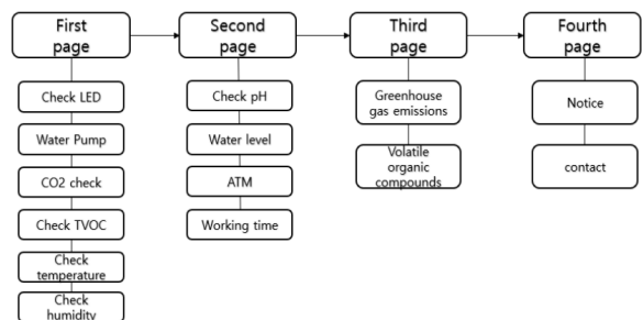
Fig. 9. Plant cultivation user interface
