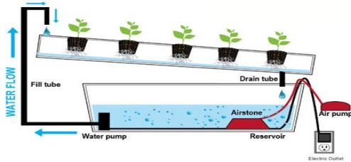
Fig. 3. Thin film hydroponic cultivation system
