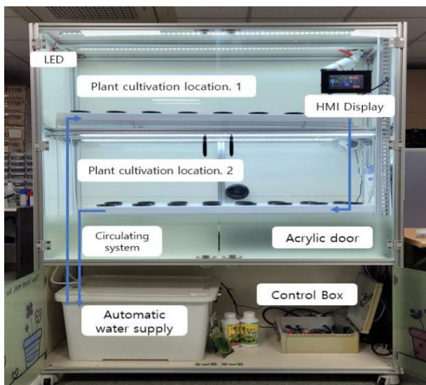
Fig. 10. Implementation of a thin-film hydroponic grower
