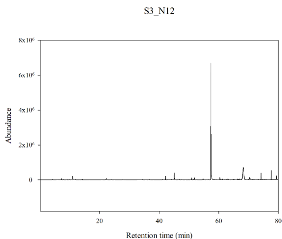
Fig. 12. Qualitative analysis of VOCs emitted from swine manure by type C feed (3rd sample). VOCs, volatile organic compounds.
