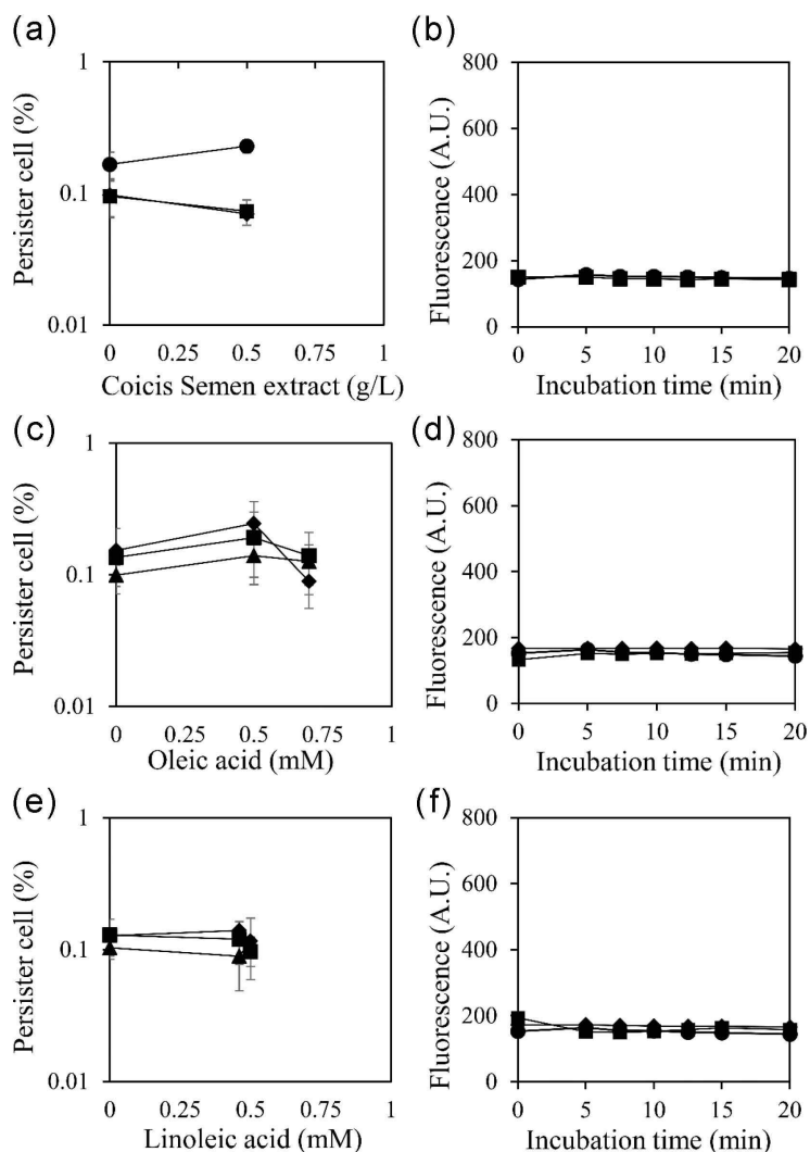
Fig. 4. Effects of Tween 80 on the reduction of persister cell and increases in cell membrane permeability in response to Coicis Semen extract, oleic acid, and linoleic acid. Changes in persister cells (a, c, and e) and permeability of Staphylococcus aureus cell membranes (b, d, and f) in response to Coicis Semen extract (a and b), oleic acid (c and d), and linoleic acid (e and f) co-administered with 1% Tween 80. Changes in persister cell numbers (a, c, and e) were then examined in cells treated with 20 mg/L of ciprofloxacin (■), 2.5 mg/L of oxacillin (◆), and 80 mg/L of tobramycin (▲). Cell membrane permeability was evaluated under the following treatments: Coicis Semen extract (b) at 0.5 g/L (■) compared to the untreated control (●), oleic acid (d) at 0.5 mM (■) and 0.7 mM (◆) compared to the untreated control (●), and linoleic acid at 0.46 mM (◆) and 0.5 mM (■) compared to the untreated control (●). The experiment was conducted in triplicate.
