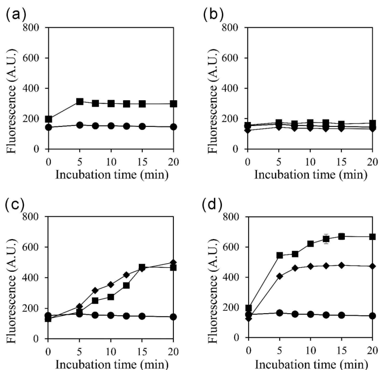
Fig. 3. Cell membrane permeability changes in response to Coicis Semen extract and its constituent fatty acids. Staphylococcus aureus cells were treated with Coicis Semen extract (a), palmitic acid (b), oleic acid (c), and linoleic acid (d), and the cell membrane permeability was measured via fluorescence. The following treatments were examined: Coicis Semen extract (a) at 0.5 g/L (■) compared to the untreated control (●), palmitic acid (b) at 0.21 mM (◆) and 0.5 mM (■) compared to the untreated control (●), oleic acid (c) at 0.5 mM (■) and 0.7 mM (◆) compared to the untreated control (●), and linoleic acid at 0.46 mM (◆) and 0.5 mM (■) compared to the untreated control (●). The experiment was conducted in triplicate.
