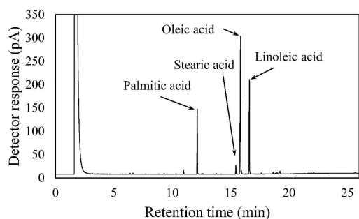
Fig. 2. Compositional analysis of ethanol extract of Coicis Semen using gas chromatography. The ethanol extract of Coicis Semen had 39.8% oleic acid, 26.0% linoleic acid, 11.0% palmitic acid, and 0.7% stearic acid. The content in the extract was calculated using the results of gas chromatography analysis with standard chemicals for analysis. The retention times were 12.139 min for palmitic acid, 15.443 min for stearic acid, 15.840 min for oleic acid, and 16.601 min for linoleic acid.
