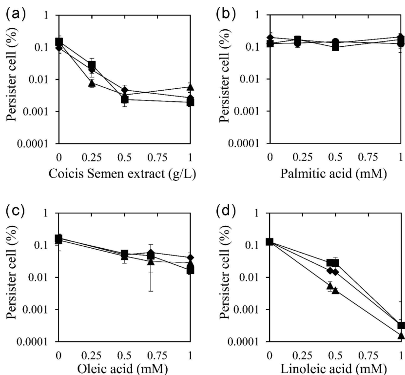
Fig. 1. Reduction in Staphylococcus aureus persister cells in response to the Coicis Semen extract and its constituent fatty acids. Coicis Semen extract (a), palmitic acid (b), oleic acid (c), and linoleic acid (d) were co-administered along with three antibiotics [20 mg/L of ciprofloxacin (■), 2.5 mg/L of oxacillin (◆), and 80 mg/L of tobramycin (▲)] to observe changes in the number of persister cells. The experiment was conducted in triplicate.
