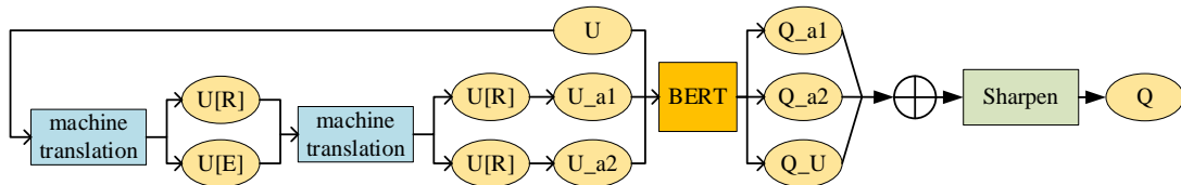
Fig. 6. Pseudo-label generation of unlabeled data.
