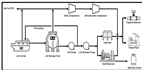
Fig. 1. Concept of liquid hydrogen receiving terminal
