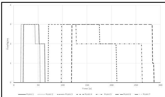
Fig. 6. Flow change in pipes according to cooldown time
