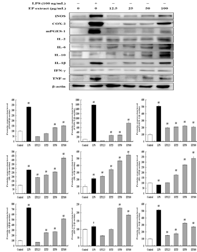
Fig. 4. Effects of Echinacea purpurea extracts on inflammatory cytokines in RAW264.7 cells. RAW264.7 cells were treated with EP extracts (12.5, 25, 50, or 100 μg/mL) or LPS (100 ng/mL) for 24 h. Protein expression was analyzed by western blot using specific antibodies. β-actin was used as controls. The data presented are the mean ± standard deviation of three independent experiments and differences between the mean values. #P < 0.05, ##P < 0.01 vs. control group
