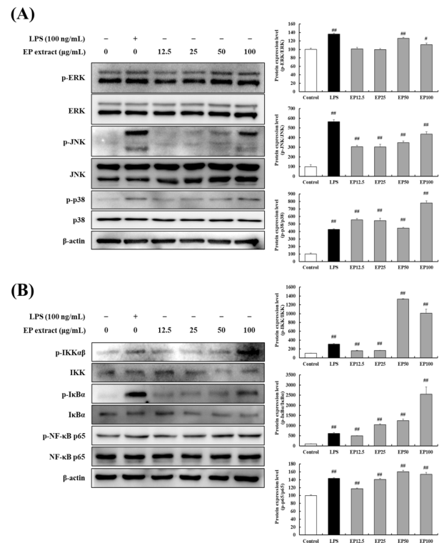
Fig. 5. Effects of Echinacea purpurea extracts on the MAPK and NF-κB pathway in RAW264.7 cells. RAW264.7 cells were treated with EP extracts (12.5, 25, 50, or 100 μg/mL) or LPS (100 ng/mL) for 24 h. Protein expression was analyzed by western blot using specific antibodies. (A) Effects of EP extracts on the MAPK pathway in RAW264.7 cells. ERK, JNK, or p38 were used as controls. (B) Effects of EP extracts on the NF-κB pathway in RAW264.7 cells. IKK, IκBα, or NF-κB p65 were used as controls. The data presented are the mean ± standard deviation of three independent experiments and differences between mean values. #P < 0.05, ##P < 0.01 vs. control group.
