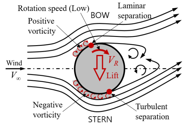
(b) Negative Magnus effect
