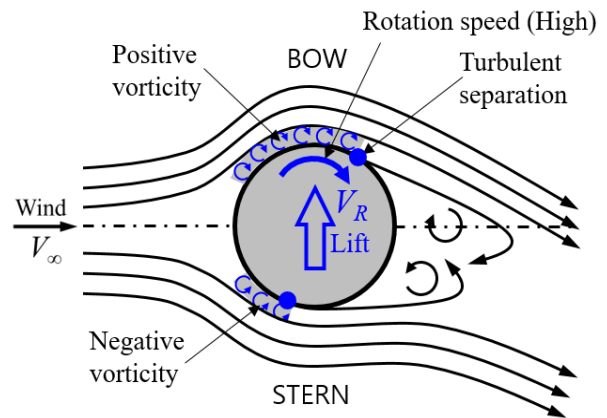
(a) Positive Magnus effect
