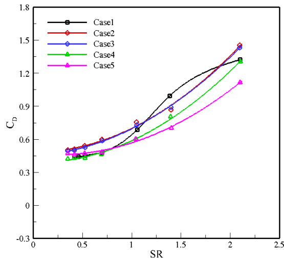
Fig. 10 Drag coefficient vs SR
