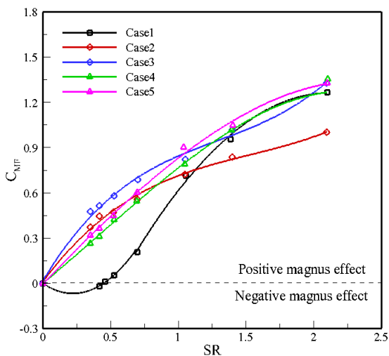
Fig. 14 Magnus force coefficient vs SR
