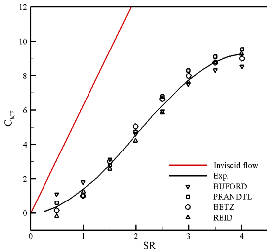
Fig. 5 Magnus force coefficient (Buford, 1954)
