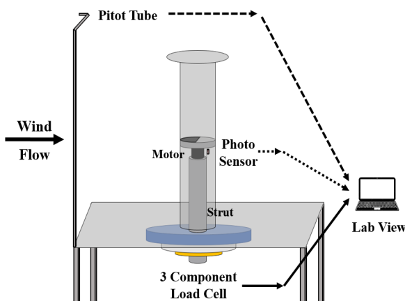
Fig. 4 Schematic view of the test-setup
