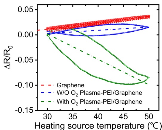
Fig. 5. Resistance change as a function of temperature for the three different cases: graphene (Red), PEI coating on graphene without O_2 plasma (Blue), and PEI coating on graphene after O_2 plasma (Green), respectively
