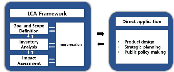
Fig. 3. LCA Framework
