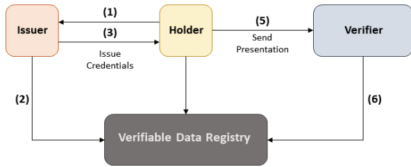
Fig. 1. Verifiable Credential Issuance Process
