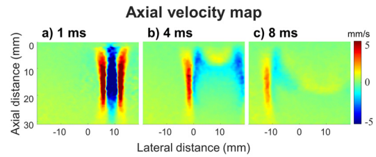
Fig. 7. (Color available online) In vitro axial velocity map results in the homogeneous region of the elasticity phantom at (a) 1 ms, (b) 4 ms, (c) 8 ms.
