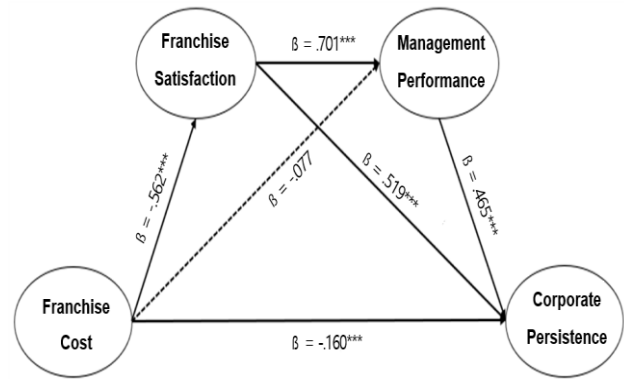
Figure 2: Path coefficient test (standardization)
