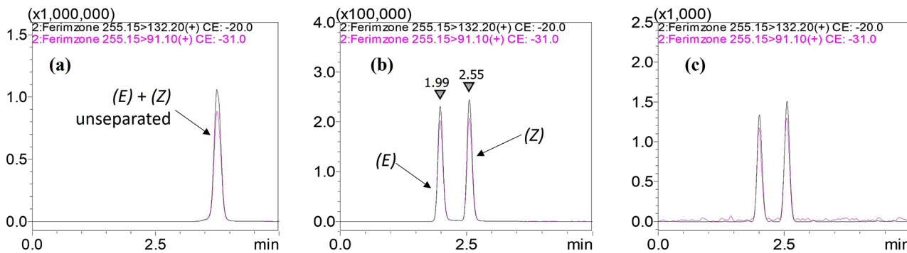
Fig. 2. Chromatograms for the comparative analysis of peak separation for ferimzone Z and E stereoisomers (100 ng/mL each) on (a) Kinetex (2.6 \mu\text{m} , 3 \times 100 mm) and (b) Cadenza columns (3 \mu\text{m} , 2 \times 150 mm), and (c) chromatogram at instrumental limit of quantitation (ILOQ; 1.25 ng/mL) using Cadenza.
