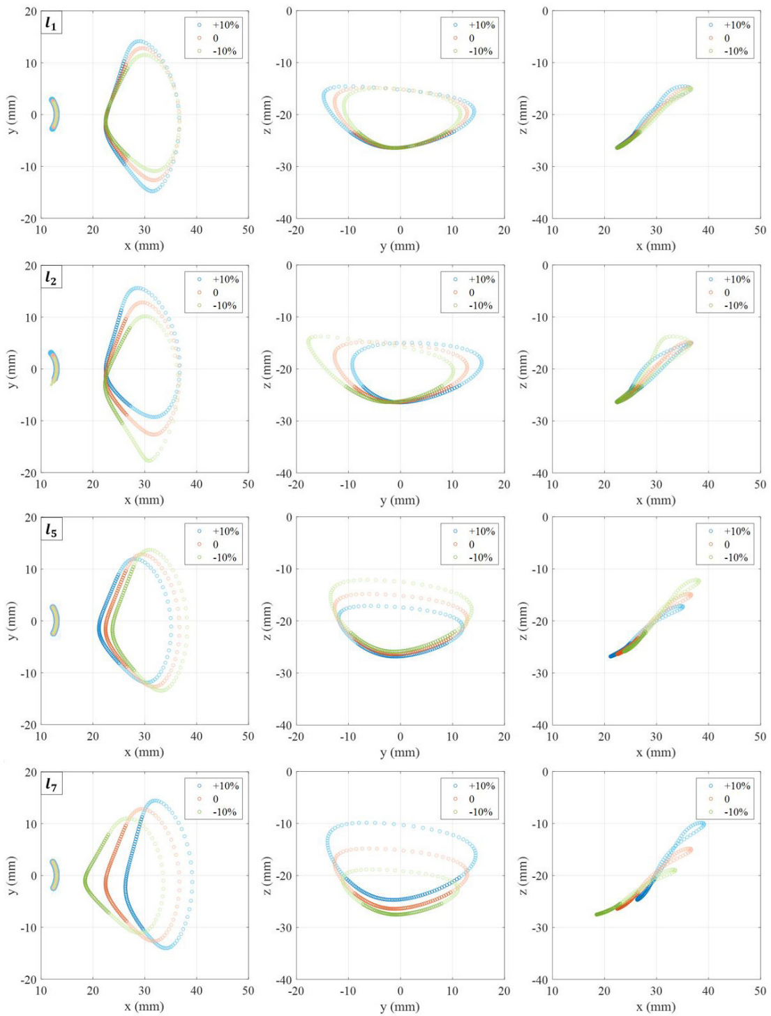
[Fig. 6] The resultant foot trajectory of the linkage while changing the design parameter ( l_1, l_2, l_5, l_7 ) in xy, yz, and xz-plane. Only one variable was changed at once. Orange points are the result of trajectory with same variable values used for [Fig. 4], and blue points are when the length of the link was increased 10%, and green points are when the length of the link was decreased 10%
