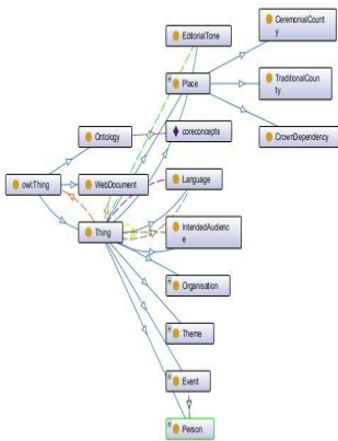
Fig 8. BCCore Concept ontology from Protégé
