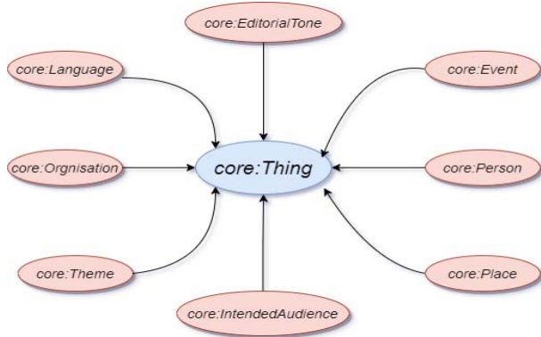
Fig7. BBC Core Concepts Ontology (BCCORE)
