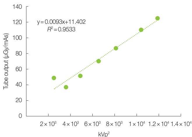
Fig. 2. Relationship between tube output and kVp^2 for the computed radiography system. kVp, kilovoltage peak; mAs, milliampere second.
