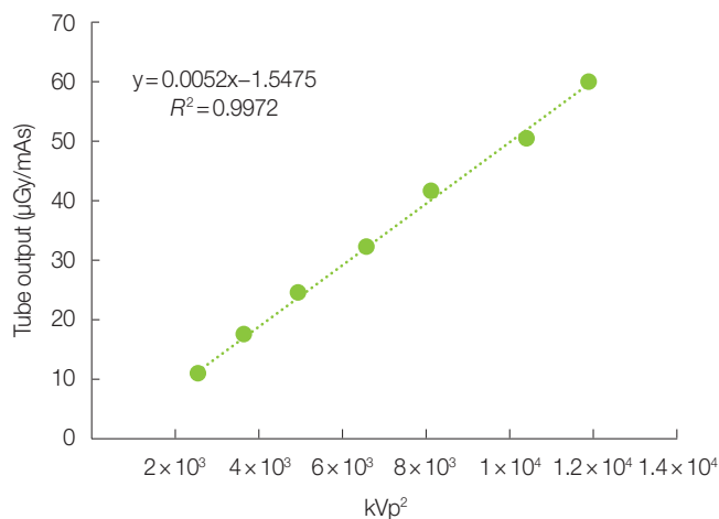
Fig. 1. Relationship between tube output and kVp^2 for the digital radiography system. kVp, kilovoltage peak; mAs, milliampere second.
