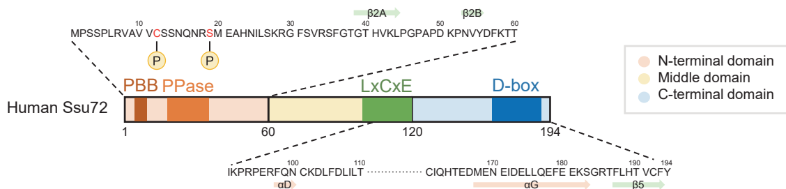
Figure 1. Schematic representation of human Ssu72 phosphatase domain structures. The Ssu72 domain comprises N-terminal (1–60), middle (61–120) or C-terminal (129–194) domains. Ssu72 possesses three structural features that distinguish it from low-molecular-mass phosphotyrosine protein phosphatases: 1) β2A and β2B, 2) αD helix, and 3) an extra helix (αG) and a β-strand (β5). Additionally, the Ssu72 protein forms functional motifs, such as PBB, D-box, and LxCxE domains, and contains a PPase domain inside. PBB, Polo-box binding; PPase, phosphatase.
