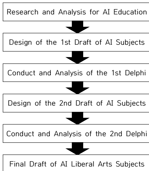
Fig. 1. Research Process
