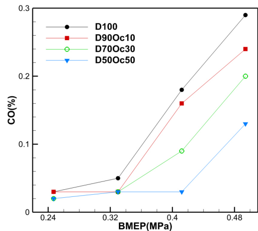
Fig. 7. Variation of CO with BMEP
