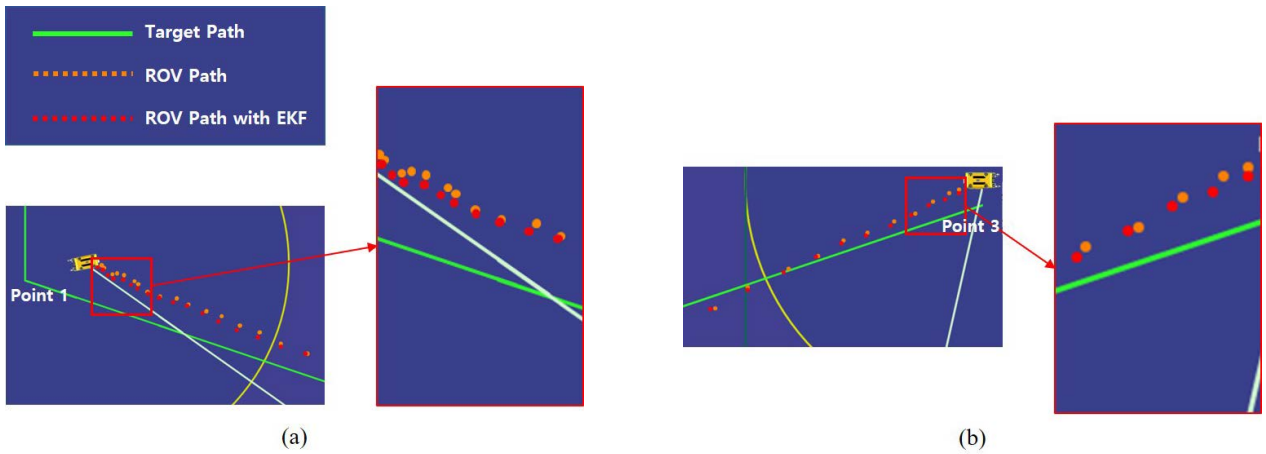
Fig. 6. ROV path with and without EKF: (a) Target point 1 of path 3 (b) Target point 3 of path 3.
