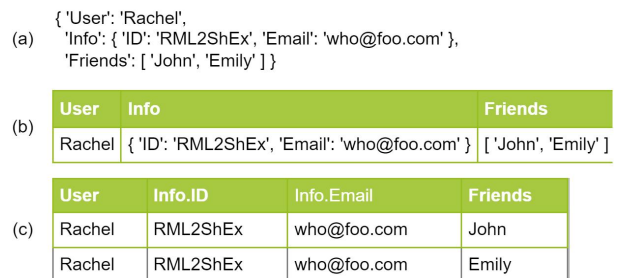
Fig. 4. Example of Flattening for JSON Data Set
