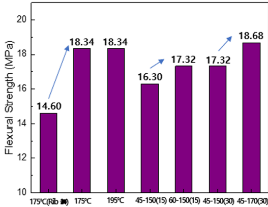
Fig. 3. Flexural strength of CFRP rebar
