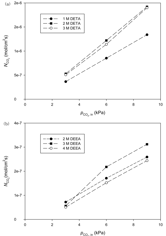
Fig. 2. Plot of CO 2 flux vs. CO 2 partial pressure: (a) DETA, (b) DEEA.
