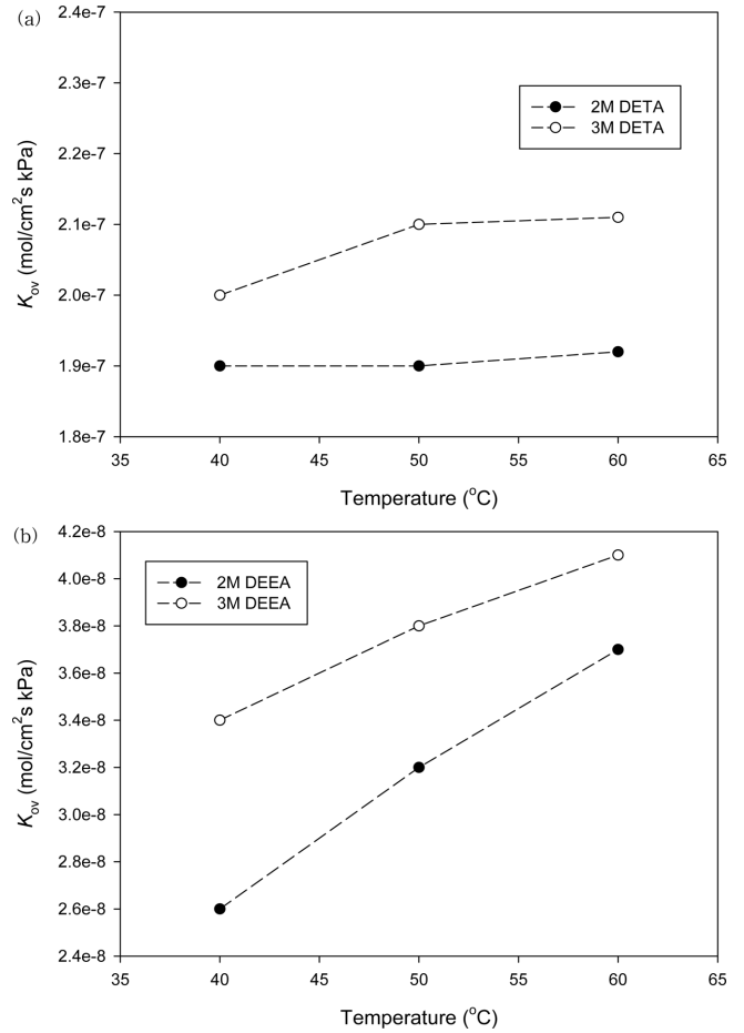
Fig. 4. Effect of the operating temperature on the overall mass transfer coefficients. (a) DETA; (b) DEEA.
