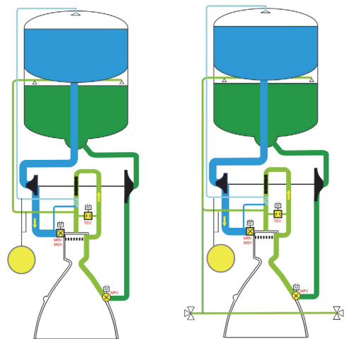
Fig. 8 Upper stage propulsion systems.
