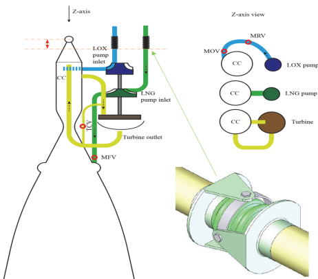
Fig. 7 Engine layout and interfaces.
