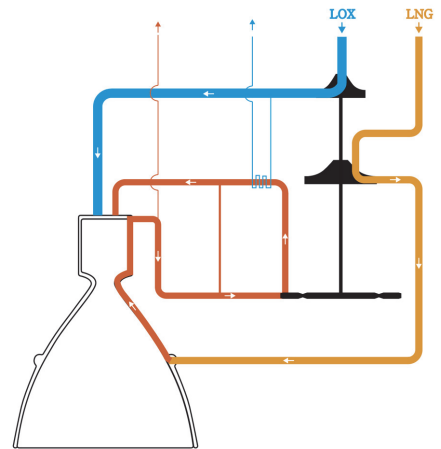
Fig. 2 Full expander cycle.
