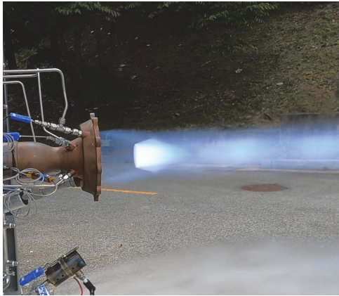
Fig. 9 Hot fire test of 1-tonf class 3D printed Methane thrust chamber [19].
