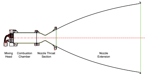
Fig. 4 Geometrical shape of Thrust chamber.
