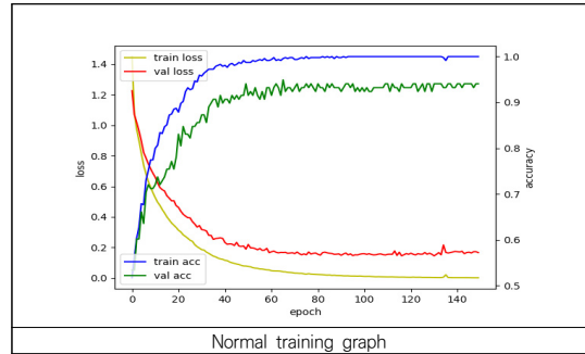
[Fig. 3] Training graphs for model verification
