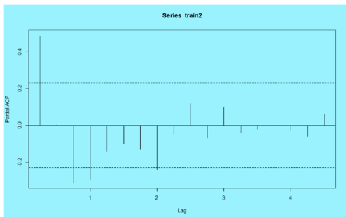
Fig 3. Partial Auto Correlation Function Plot
