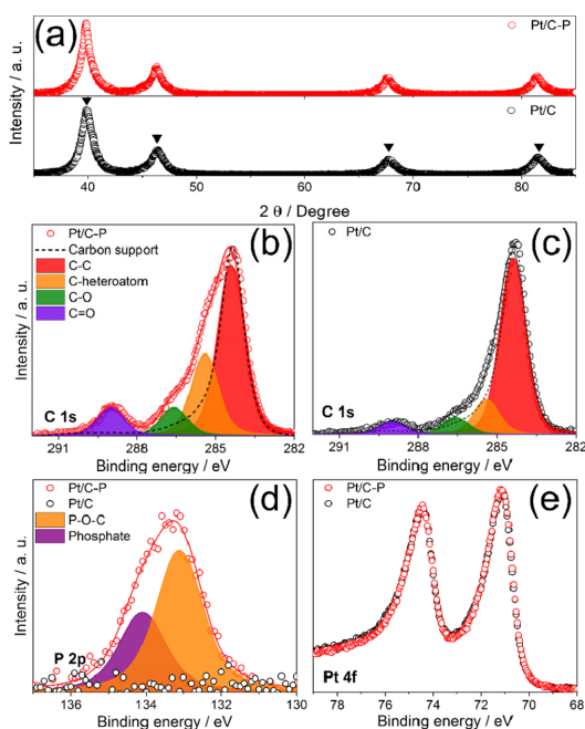
Fig. 2. (a) XRD patterns of Pt/C-P and Pt/C ( \blacktriangledown =FCC Pt). XPS spectra in C 1s orbital of (b) Pt/C-P and (c) Pt/C ( \circ : raw data, \text{—} : fitted data). XPS spectra of Pt/C-P and Pt/C in (d) P 2p orbital and (e) Pt 4f orbital.
