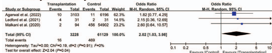
Fig. 4. Forest plot showing (A) the readmission rate, and (B) 90-day mortality rate for hip arthroplasty following solid organ transplantation. CI: confidence interval.
