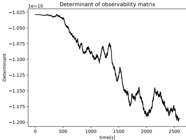
Fig. 6. Det ( M_0 ) graph.
