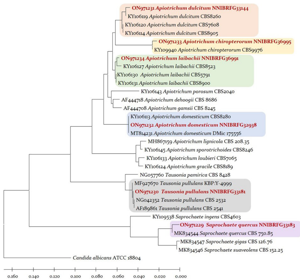
Fig. 1. Phylogenetic tree of unrecorded yeasts isolated from freshwater and related species based on a Neighbor-joining analysis of the nucleotides sequences of large subunit 26S ribosomal DNA D1/D2 region, using MEGA-X. The sequences of Candida albicans was used as outgroup. The unrecorded yeasts are shown in bold and red.
