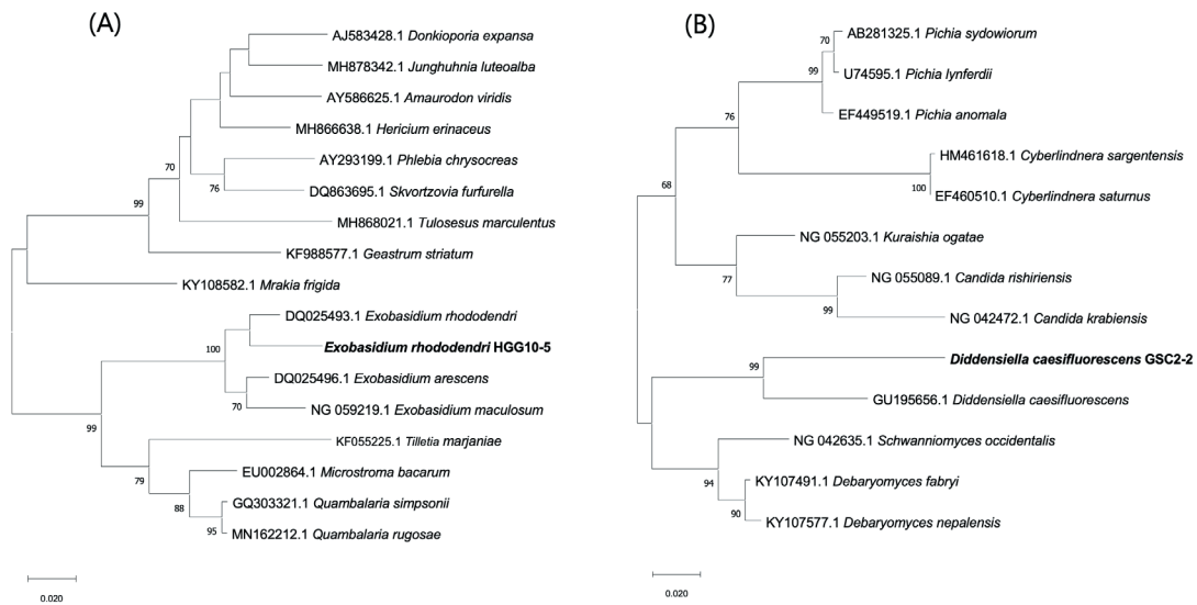
Fig. 3. Phylogenetic tree of the unrecorded yeasts, Exobasidium rhododendri HGG10-5 (A) and Diddensiella caesifluorescens GSC2-2 (B) isolated from waters and soils of Haegeumgang in southern sea and Geumsancheon in Geumgang upstream of Korea, based on the nucleotide sequences of large subunit 26S ribosomal DNA D1/D2 region. The tree was generated by the neighbor-joining method, using MEGA X.
