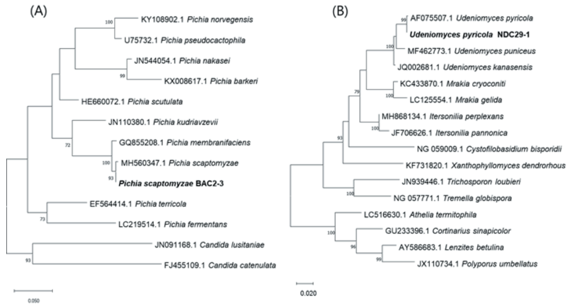
Fig. 2. Phylogenetic tree of the unrecorded yeasts, Pichia scaptomyzae BAC2-3 (A) and Udeniomyces pyricola NDC29-1(B) isolated from waters and soils of Namdaecheon in Geumgang upstream of Korea, based on the nucleotide sequences of large subunit 26S ribosomal DNA D1/D2 region. The tree was generated by the neighbor-joining method, using MEGA X.
