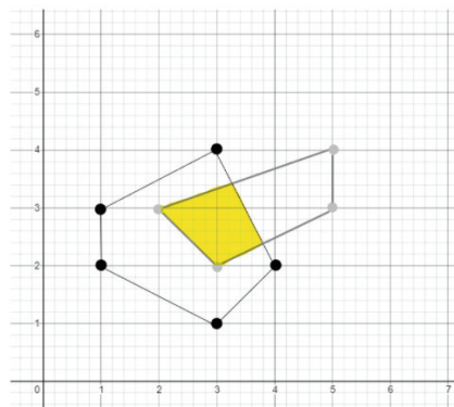
Fig. 6. Calculate area of intersection of n-gon.
