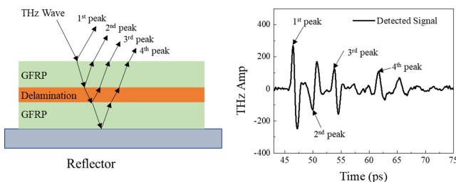
Fig. 1. Schematic of defect inspection through THz system
