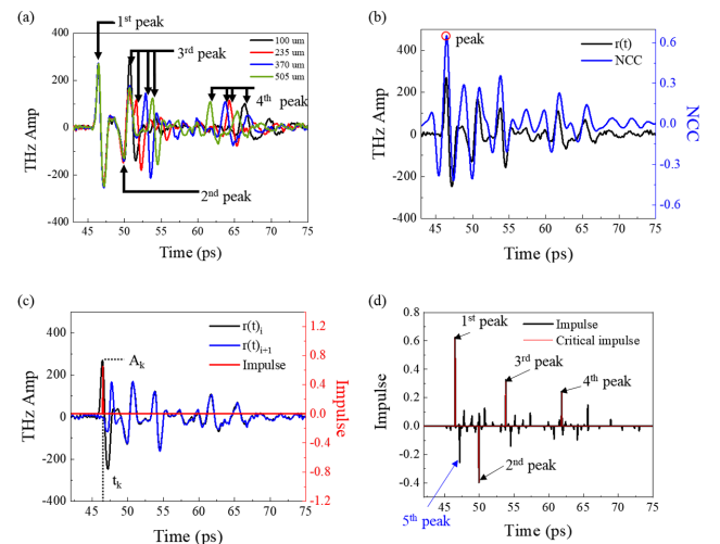
Fig. 4. (a) THz signals measured by reflection mode with respect to the defect size, (b) NCC result of THz incident and detected signal, (c) extracted impulse and the signal after impulse extraction, (d) extracted impulse function and critical impulses
