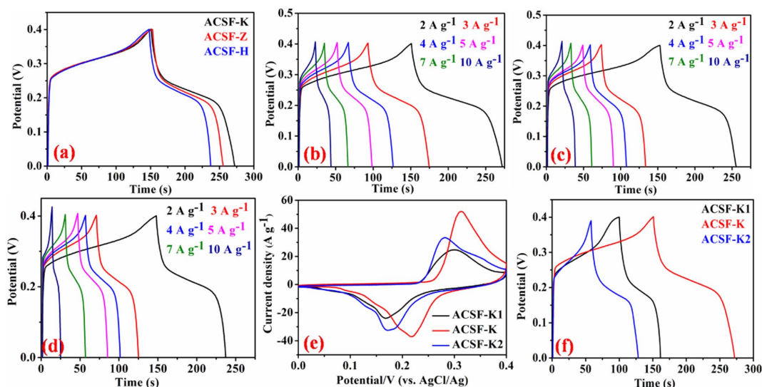
Fig. 4. (a) Comparable GCD curves (b-d) GCD curves of ACSF-K, ACSF-Z and ACSF-H electrodes, respectively at different current density of 2-10 \text{A g}^{-1} (e,f) Comparable CV and GCD curves of the electrodes at different concentration of KOH
