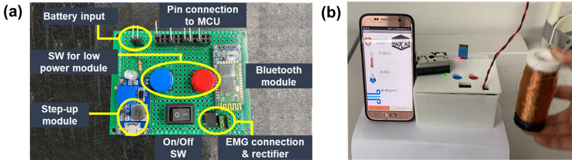
Fig. 5. (a) Sensor package composition and (b) the operation of the environmental monitoring system.
