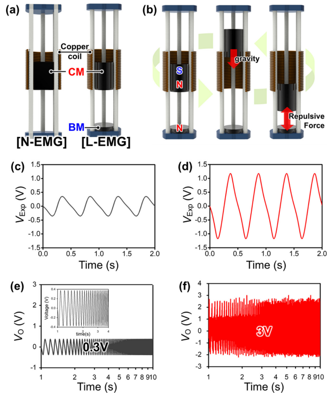
Fig. 2. (a) Comparison of the N-EMG and L-EMG and (b) the operational mechanism of the L-EMG. The output expectation ( V_{Exp} ) from the (c) N-EMG and (d) L-EMG with the COMSOL. The real voltage output ( V_0 ) from the (e) N-EMG and (f) L-EMG.
