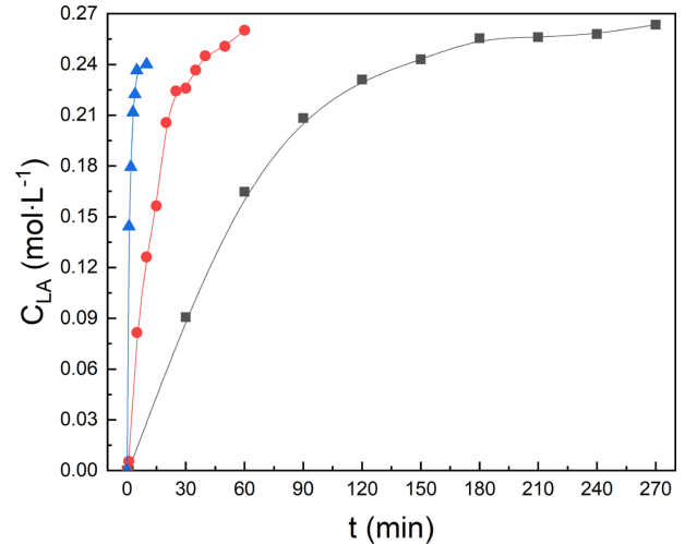
Fig. 5. Concentration of LA at different temperatures (3 wt% H_2SO_4 , X_{Glu} = 0.99 , ■ 160 °C, ● 180 °C, ▲ 200 °C).
