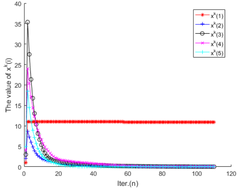
FIGURE 1. The Algorithm 3.1 with x^0 = (1, 2, 3, 4, 5)^\top , x^1 = (0, 1, -1, 2, 3)^\top , the tolerance \epsilon = 10^{-3} .
