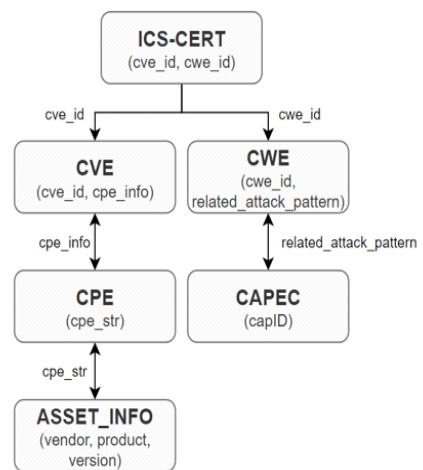
Fig. 2. Relationships between Database tables
