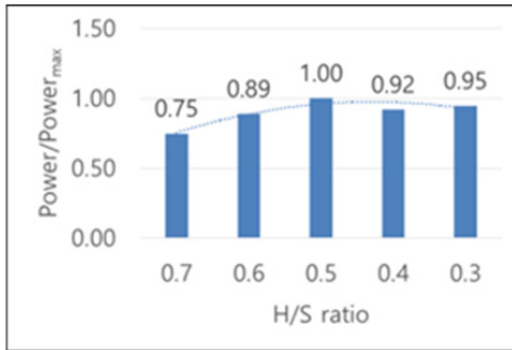
(b) Hub-to-shroud ratio
