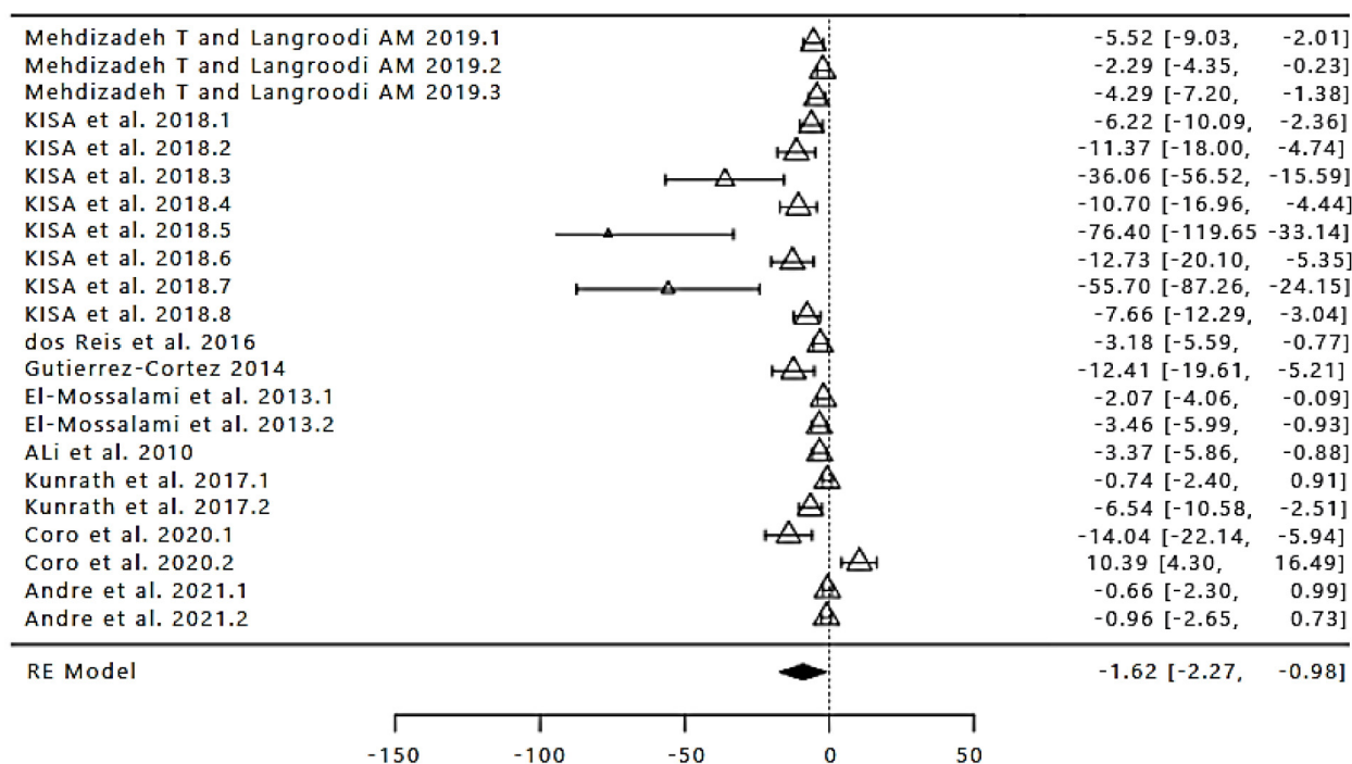
Fig. 4. Forest plot analysis of TBARs values at various concentrations of PE (propolis extract) on various livestock products using the Random Effect model. TBARs, thiobarbituric acid reactive substances.
