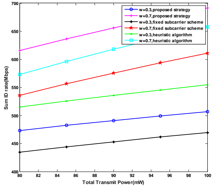
Fig. 3. The relationship between the sum ID rate and transmit power.
