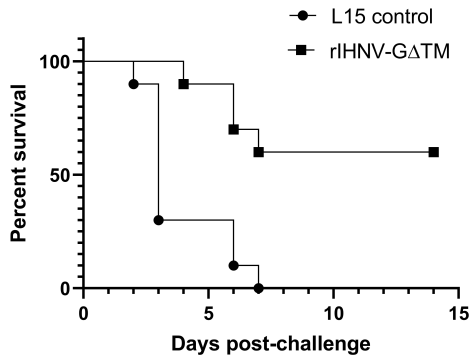
Fig. 3. Kaplan-Meier curve of survival of rainbow trout. Fish were immunized with 1.5 \times 10^2 PFU/fish of rIHNV-GΔTM or L-15 medium alone. At 3 weeks post-immunization, fish were intramuscularly challenged with 2.0 \times 10^6 PFU/fish of wild-type IHNV.
